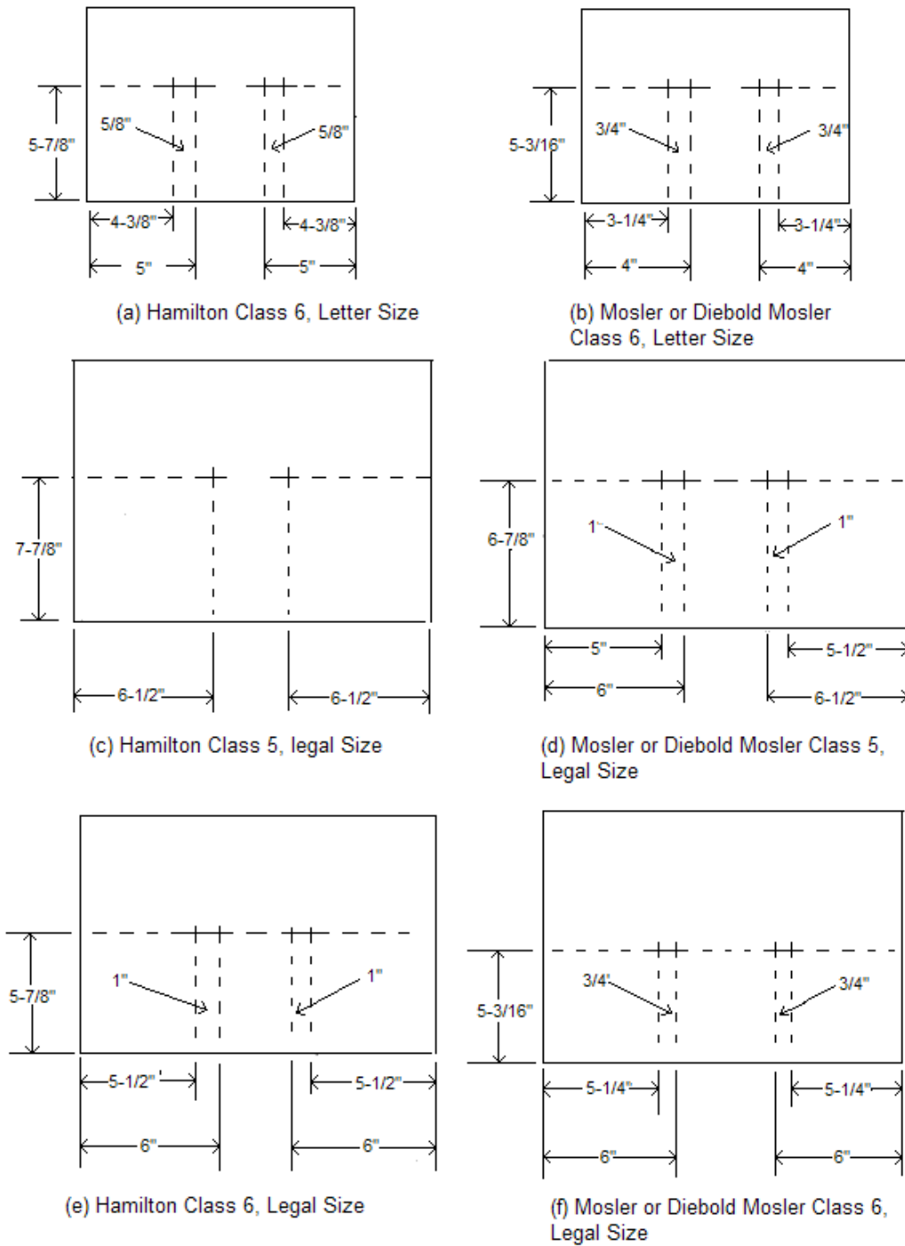
Figure 4. Classes and sizes of security containers, showing cut marks locations.
