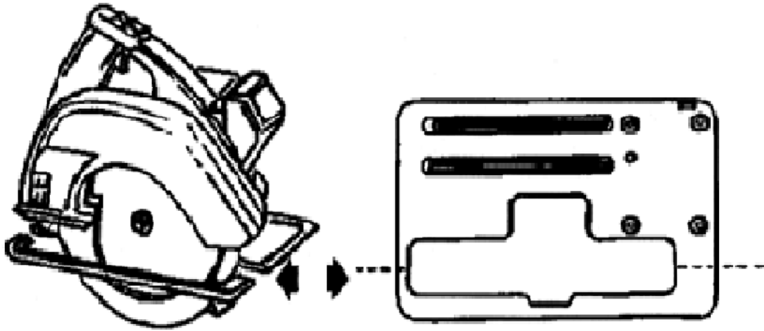
Figure 3. Builder's circular saw. Cut the foot assembly of the 10 ¼" circular saw as shown. File or grind the cut edges of the foot assembly to remove sharp edges. This size saw is necessary on Mosler or Diebold-Mosler Class 5 security files. A 7 ¼" builders circular saw is adequate for other files and does not require the modification shown above.
